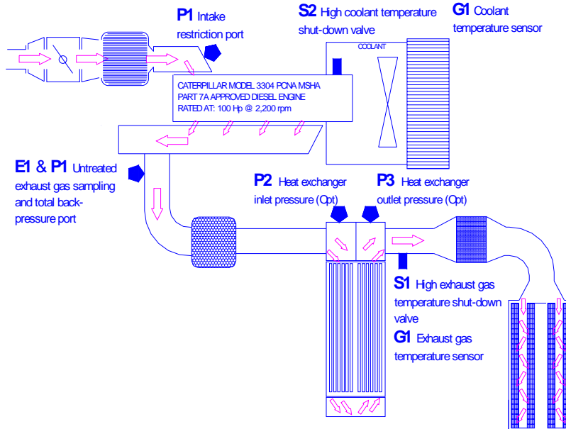
Illustration No. 4: Location of Pressure and Temperature Probes
