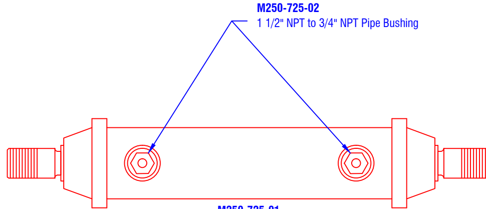
M250-725-01 OIL COOLER TOP VIEW
