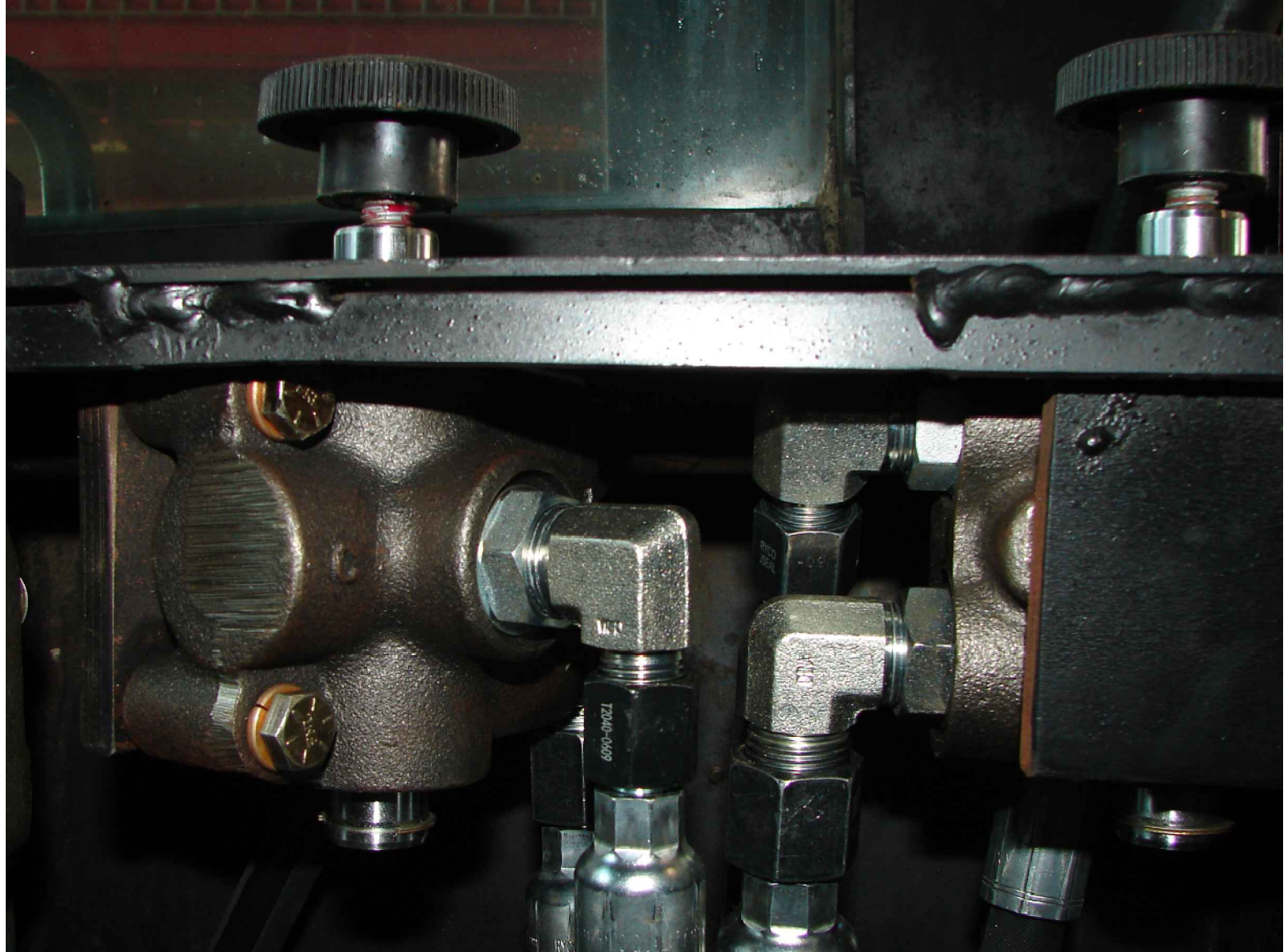
HI/LO SPEED SELECTOR & PARK BRAKE VALVE
