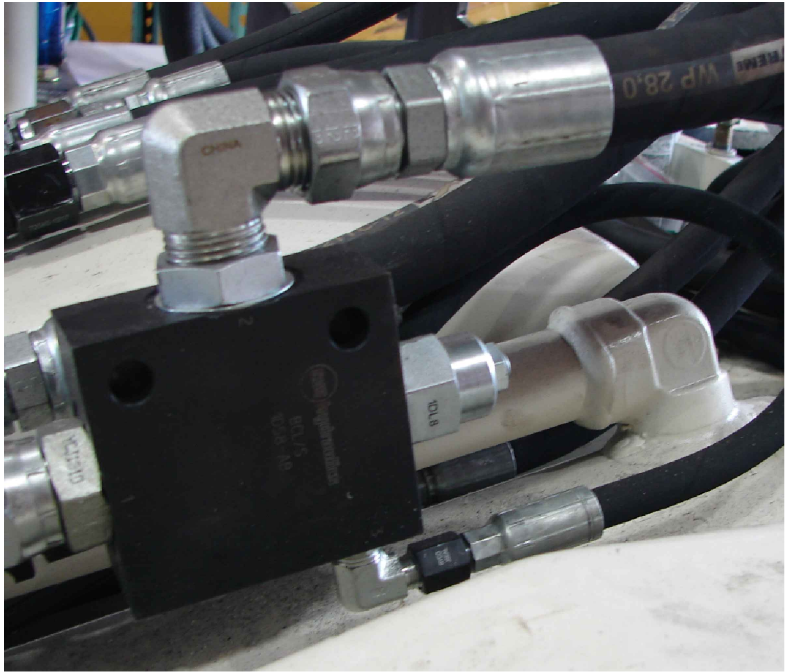
M350-506-14 CARTRIDGE, COUNTERBALNCE VALVE
