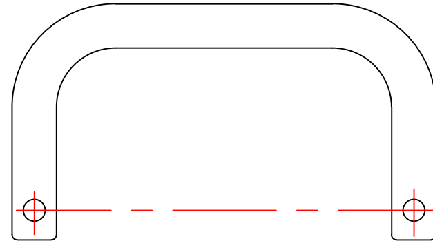
M350-233-01 Guard, Driveline, Articulation
