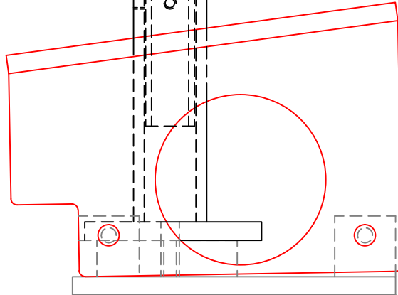
LOWER MOUNT PART OF FRONT FRAME FENDER
