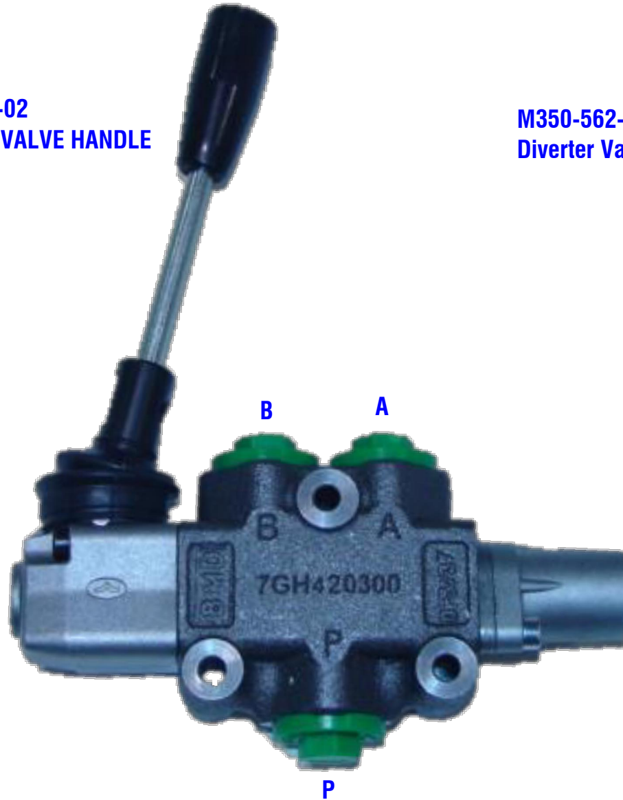
M350-562-01 DIVERTER VALVE
