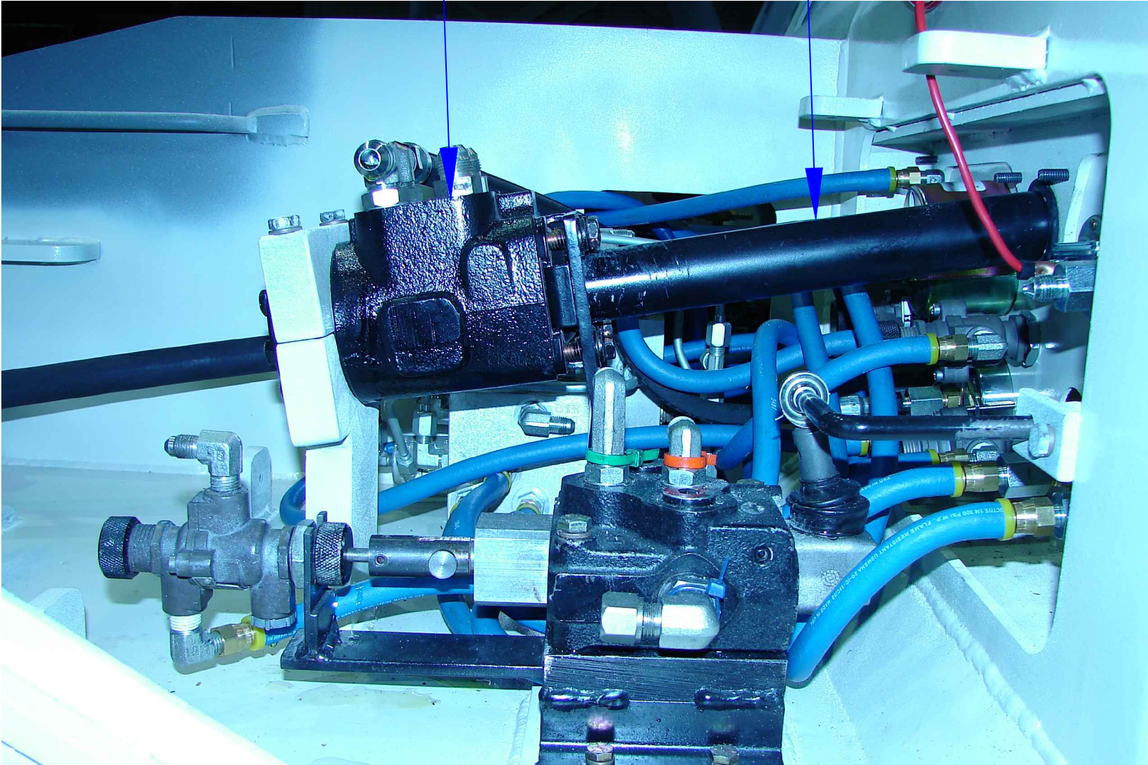
M375-521-01 COLUMN, ORBITROL STEERING
