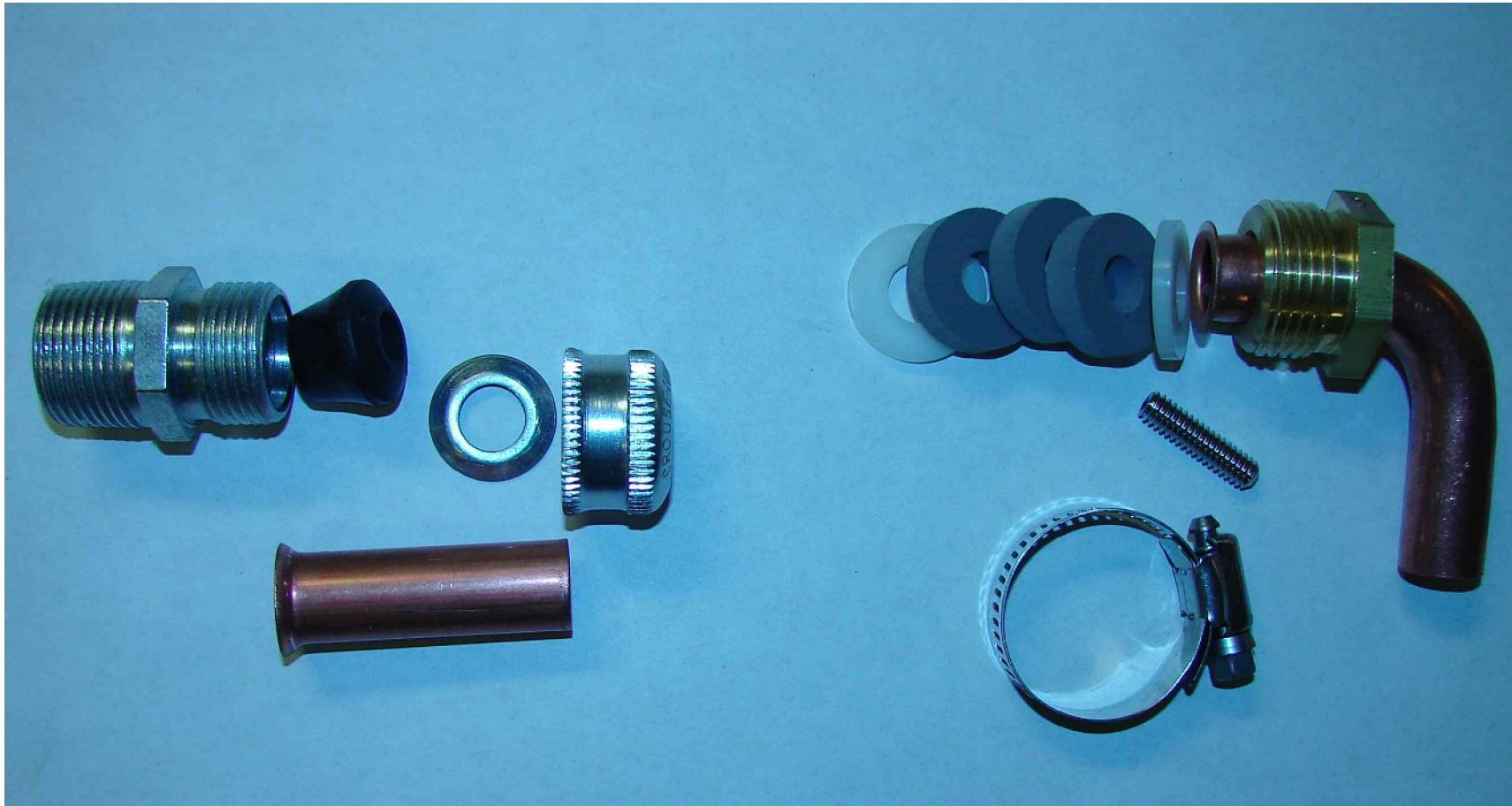
M261-570-01 CABLE GLAND ASSEMBLY Crouse Hinds style cable gland
